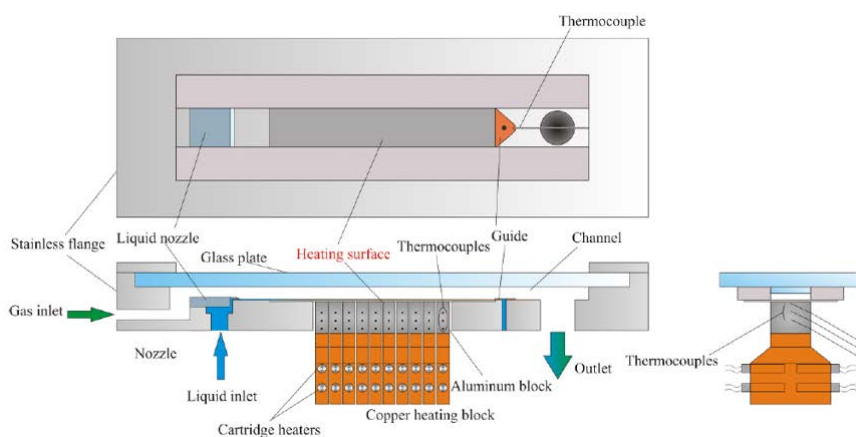
Fig. 2 Structure of test section.
