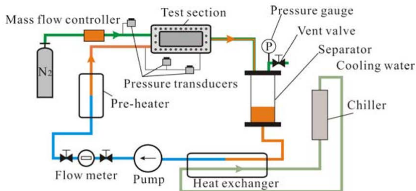
Fig. 1 Outline of test loop.
